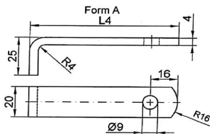
Base (part No. 3)
